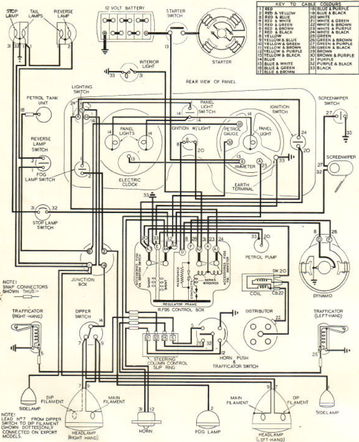
Illustration No. N.28. Diagram of the wiring system, with RF.95/2 Control Unit. (Commencing Chassis No. Y.0584.)
