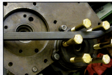
Turn the crank like this. Do NOT use your new ARP flywheel bolts for this
