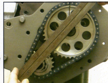
The straight edge line should go through the cam/crank shaft centers as well as the two gear 'dots'.
