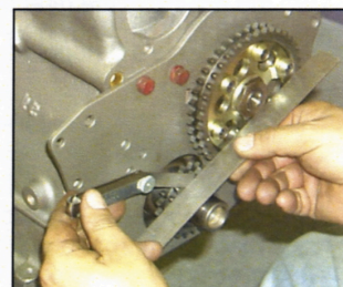
If these gears run out of line that's not good for chain life, or the gears!
