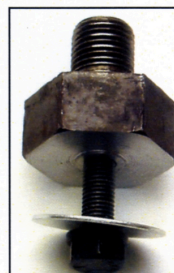
This crank bolt has a register on the front face to locate the degree wheel
