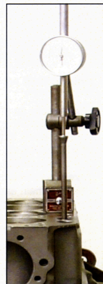
Reading lift on cylinder #1 inlet lobe. Remember this is normally the second hole from the front.
